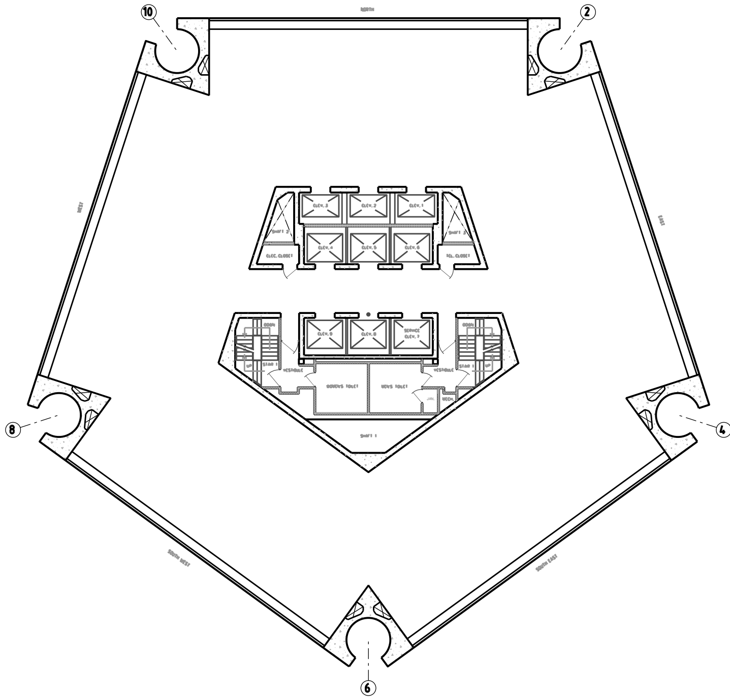
21st FLOOR CORE PLAN SCALE: 1/8" = 1'-0"
