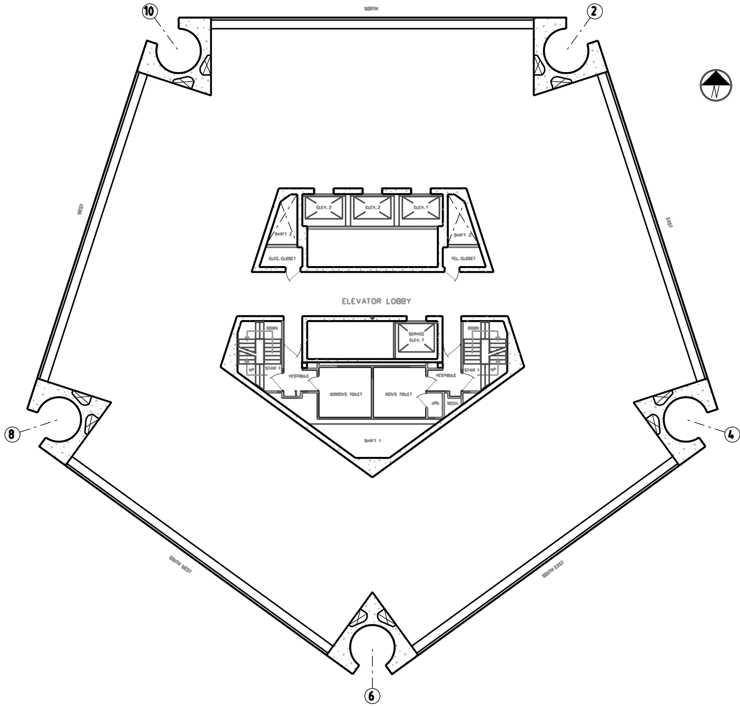
22nd FLOOR CORE PLAN SCALE: 1/8" = 1'-0"
