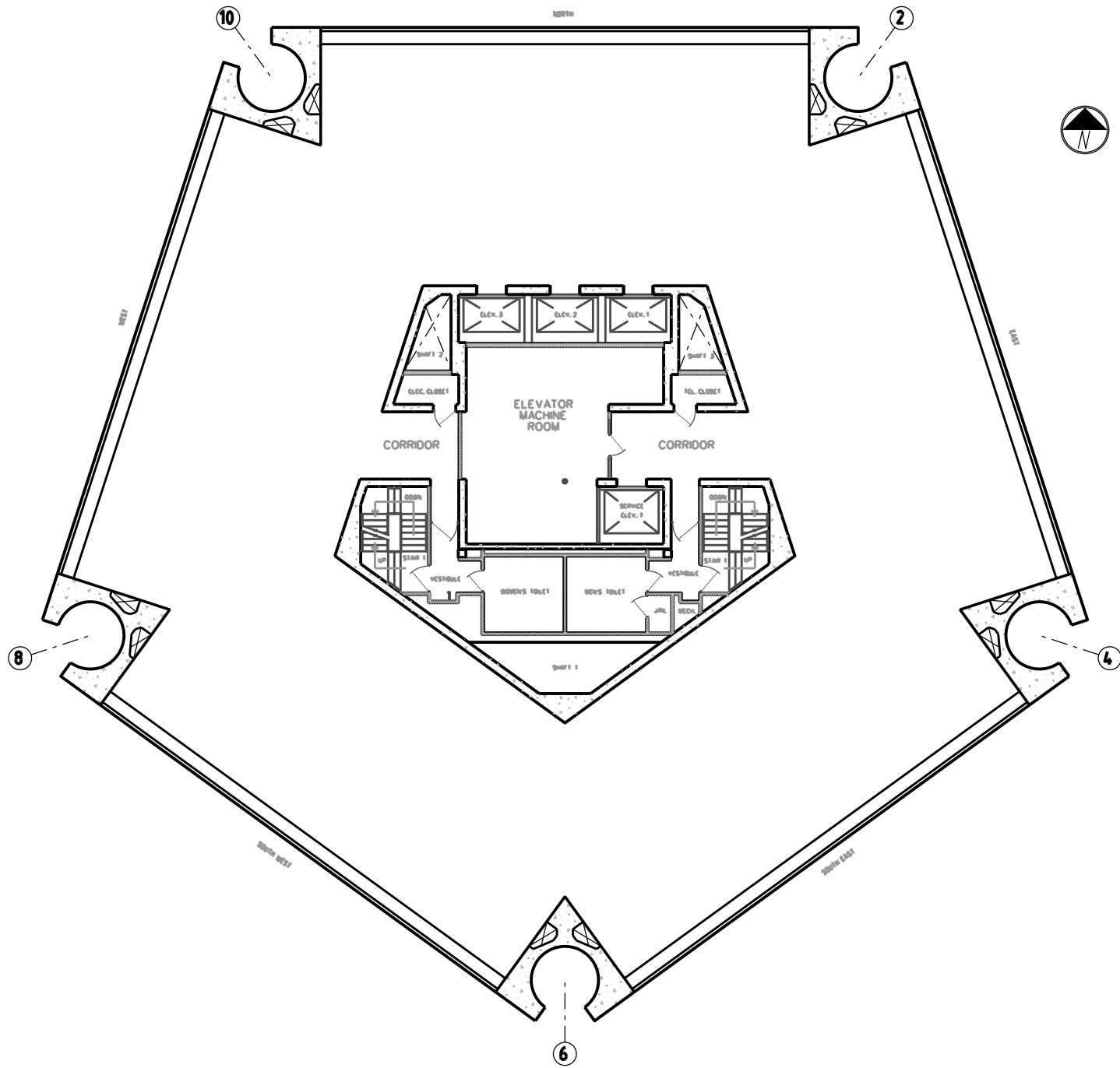
23rd FLOOR CORE PLAN SCALE: 1/8" = 1'-0"
