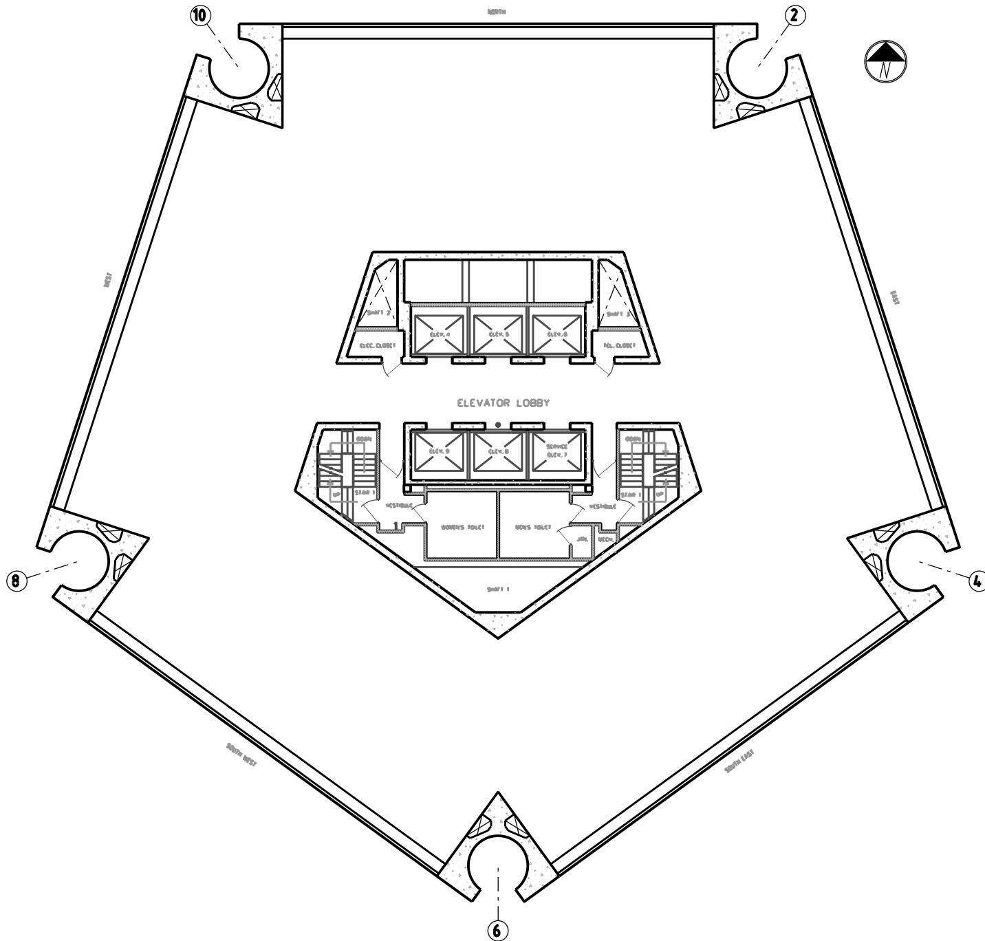
2nd - 20th FLOOR CORE PLAN SCALE: 1/8" = 1'-0"
